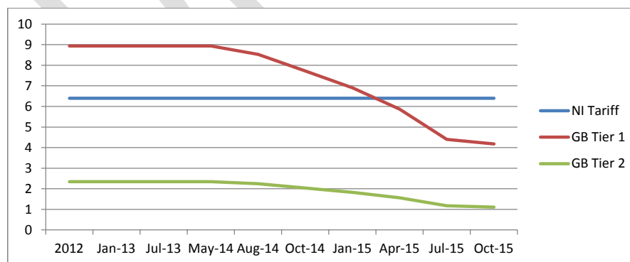
Graph 1: Comparison of Northern Ireland and GB RHI non-domestic tariffs from 2012 to 2015 in pence (based on a typical 99kw biomass boiler) *
